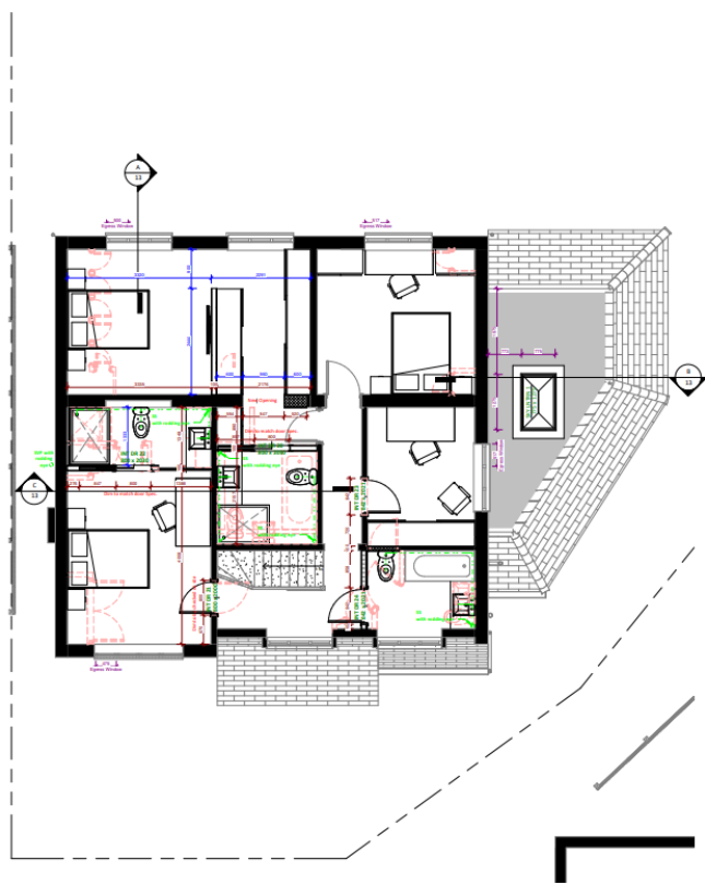
2 Proposed First Floor 1:50
