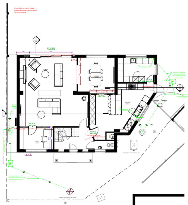
1 Proposed Ground Floor 1:50
